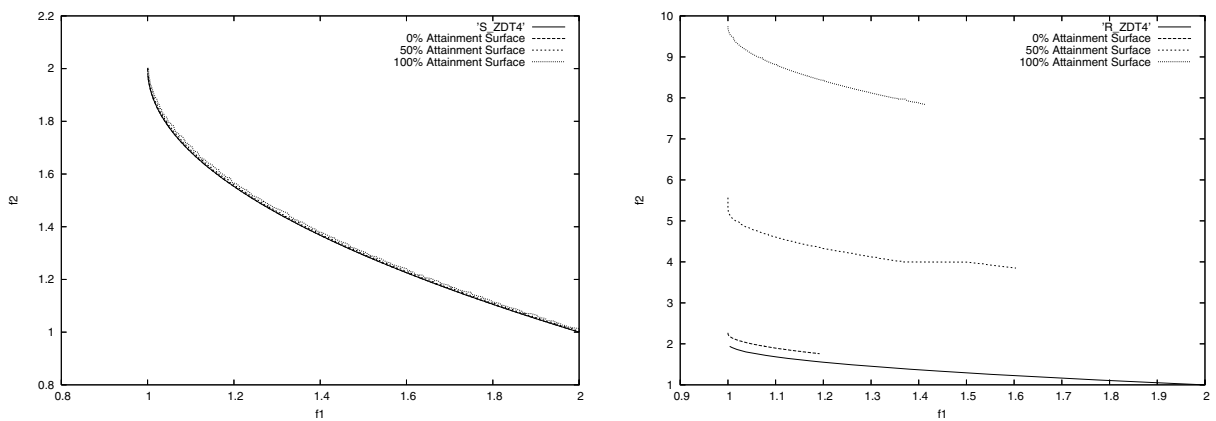
Fig. 3. Attainment plots of S_ZDT4 and R_ZDT4.
