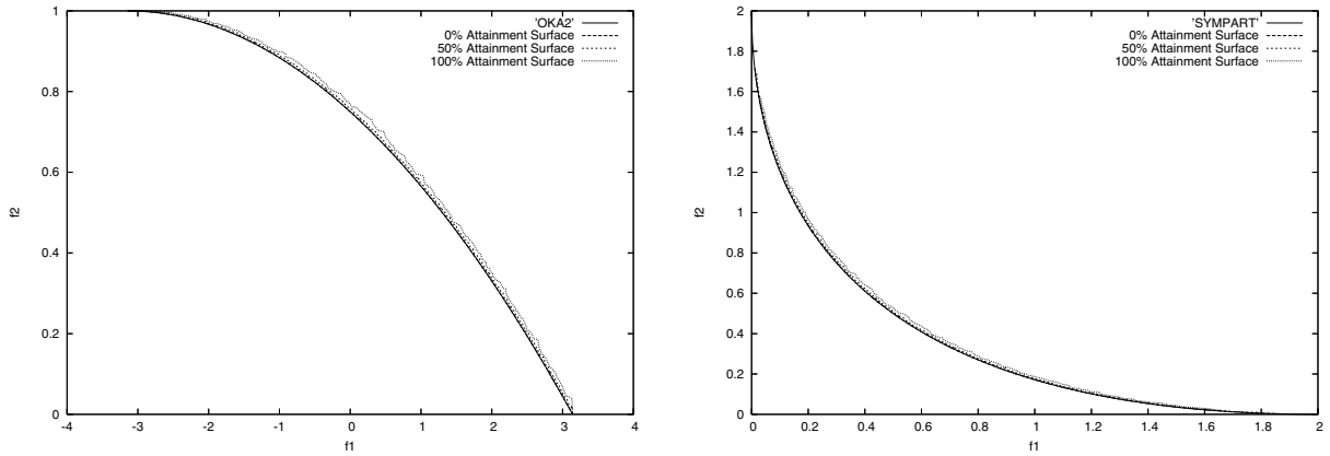
Fig. 1. Attainment plots of OKA2 and SYMPART.
