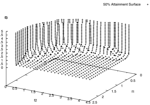
Fig. 4. Attainment plots of S_ZDT6 and WFG1_M3.
