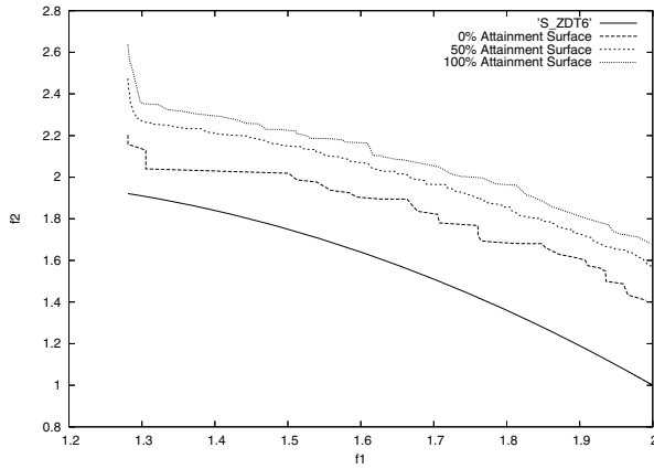
Fig. 4. Attainment plots of S_ZDT6 and WFG1_M3.
