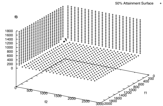
Fig. 5. Attainment surfaces of S_DTLZ2_M3 and R_DTLZ2_M3.
