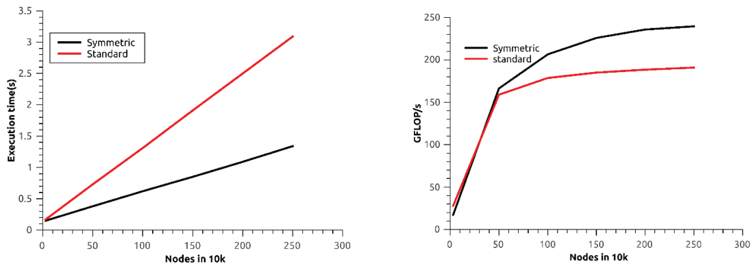
Figure 4. Wall clock time (a) and GFLOP/s count (b) for local matrix generation vs number of nodes in 10,000 in symmetric and standard versions.
