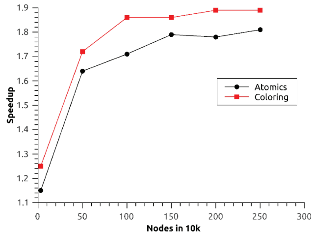
Figure 7. Comparison of speedup of symmetric version compared to atomics version with number of nodes
