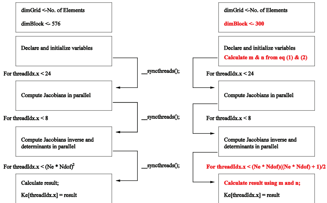
Figure 2. Flow of work in standard (left) and symmetric (right) kernel
