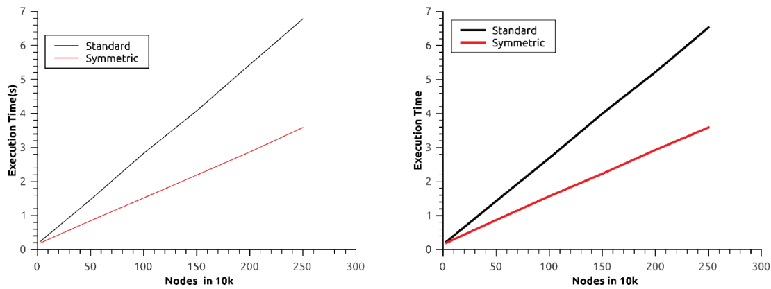
Figure 6. Wall clock time comparison for Coloring (A) and atomics (B) version with nodes in 10,000
