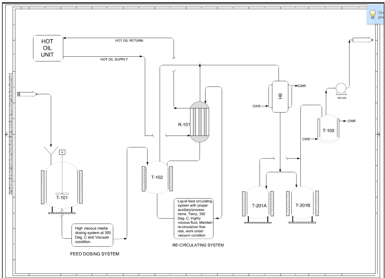
Figure 1: Process Flow Diagram of Polymerization Plant
